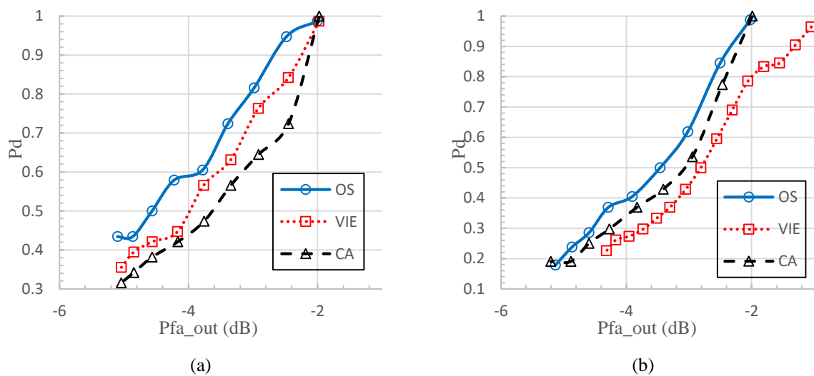
Fig. 10. ROC curves of three detection methods (a) Image 2, (b) Image 3
