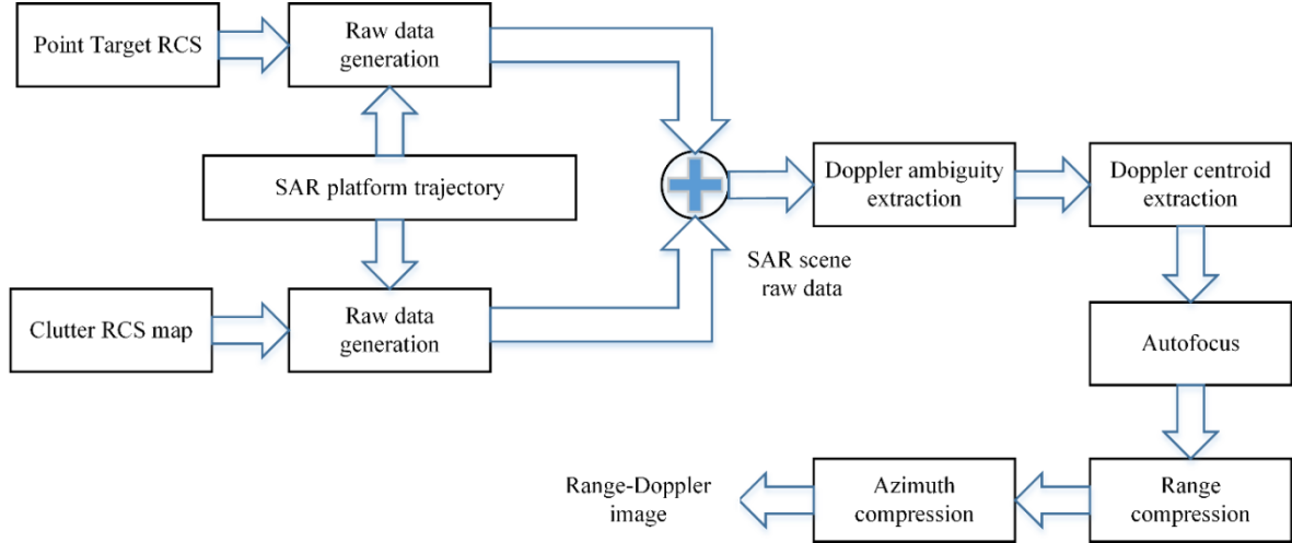
Fig. 3. SAR image simulation block diagram
