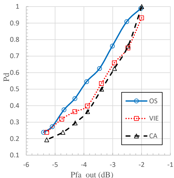
Fig. 11. ROC curve for Image 4
